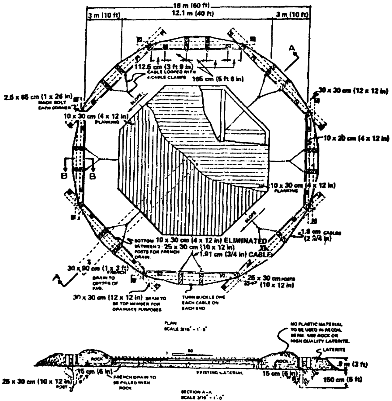
Figure 1-31. Gun pad for 8-inch or 175-mm with non-radial sleepers.
